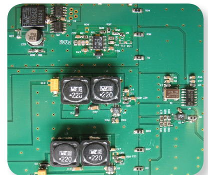
Synchronized DC/DC converters for generating different voltage levels from a battery source.
