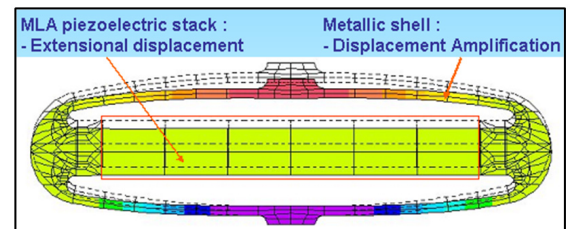
Fig. 1: APA® FEM Deformed structure.
