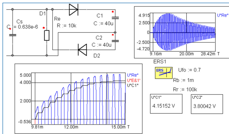
Figure 3: Simulation with electronic.
