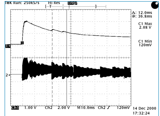
Figure 4: Output voltage, the effect of the rebounds are clearly visible.
