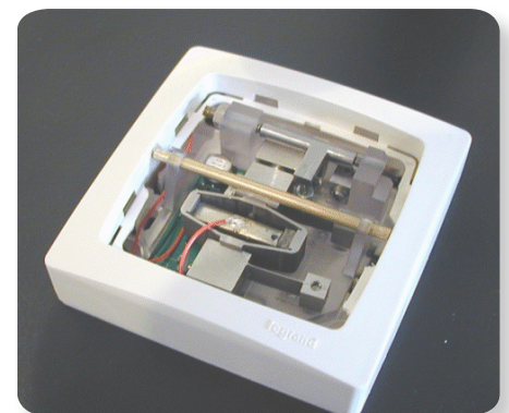
Figure 6: Complete mechanism set up in a switch (Courtesy of Legrand).
