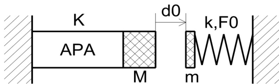
Figure 1: Scheme of the system.
