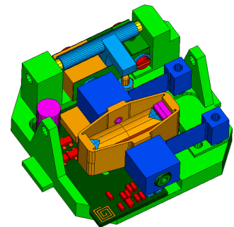
Figure 5: CAD drawing of SEH-APA 60SM.
