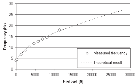
Fig.9: Measured & theoretical freq. vs Preload
