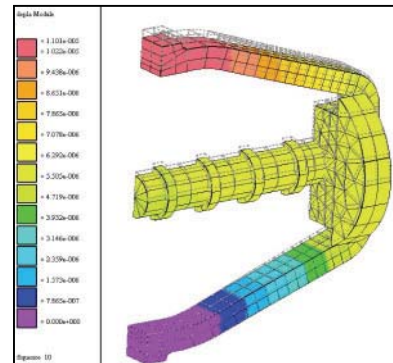
Fig. 4 : ATILA modelling of the AMA400L
