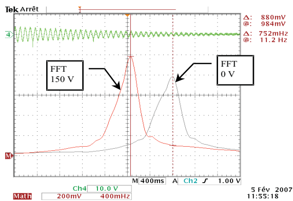
Fig.10: Frequency response of TPMA vibration speed with preload actuator on (150V) or off (0V)
