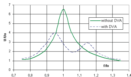
Fig.1: Effect on the frequency response of a structure due to a DVA tuned with the resonance
