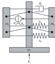
Fig.6: TPMA initial concept
