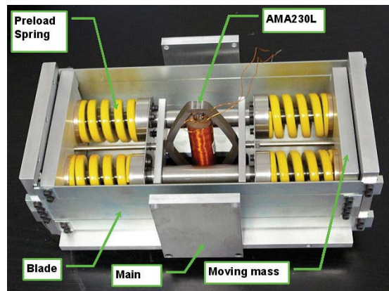
Fig.8: TPMA prototype
