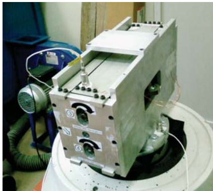
Fig.11: TPMA in vibration test set-up
