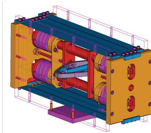
Fig.7: TPMA CAD view
