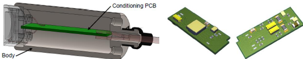
Figure 6. Micro-Switch embedded space grade conditioning PCB design
