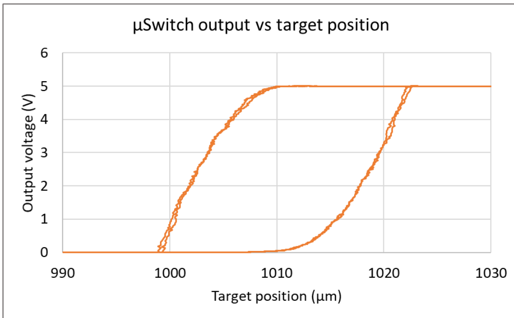
Figure 13. Sensing test results – Forward / backward Hysteresis threshold
