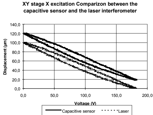
Figure 8 : Hysteresis measurement X axis excited (laser in position RX)(An offset is used for a clearer view)
