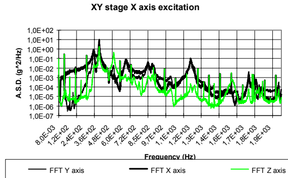
Figure 9 : A.S.D. level ( \text{g}^2/\text{Hz} ) on the X axis excitation
