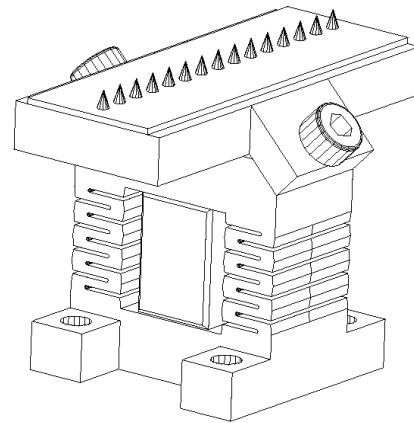
Figure 12 : Piezoelectric Z actuator supporting the needles.
