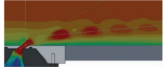
Figure 1: CFD Simulation for SJA optimization
