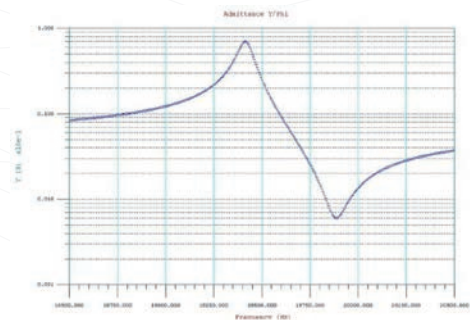
Fig. 4: Electrical admittance of a piezoelectric transducer.
