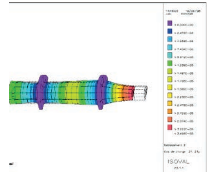
Fig. 2: Transducer simulation with ATILA.
