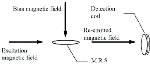
Fig. 1: Detection principle.
