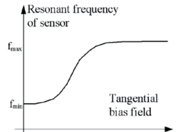
Fig. 6: f(Ht) law of L.C. M.R.S.
