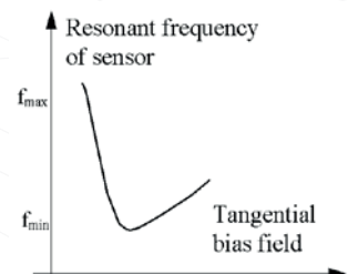
Fig. 9: f(Ht) law of magnetostrictive M.R.S.
