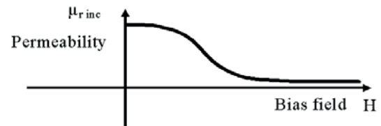
Fig. 3: Dynamic permeability versus bias field.
