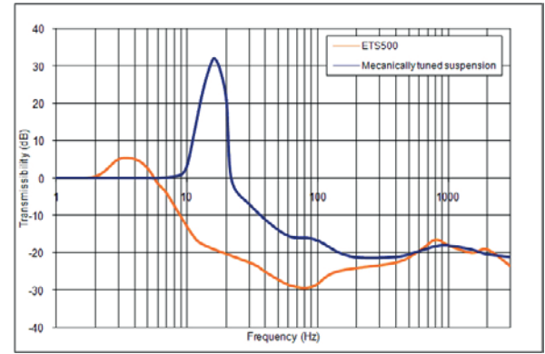
Fig. 2: Comparison of the Electrically Tuneable Suspension performances compared to a conventional passive mechanically tuned suspension performances.
