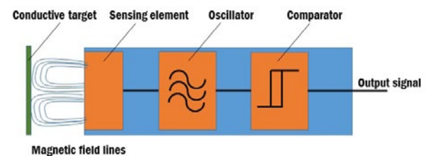
Fig. 2: Construction of the LES1000 proximity sensor
