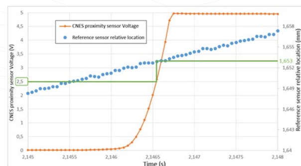
Fig. 3: Example of conductive target detection and relative output voltage
